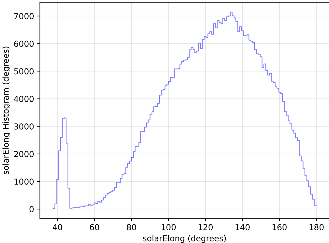
ddf_loaded_half_fl4_v3.4_10yrs All sky r band: solarElong Histogram
