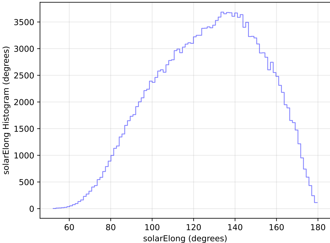
ddf_loaded_half_fl4_v3.4_10yrs All sky g band: solarElong Histogram
