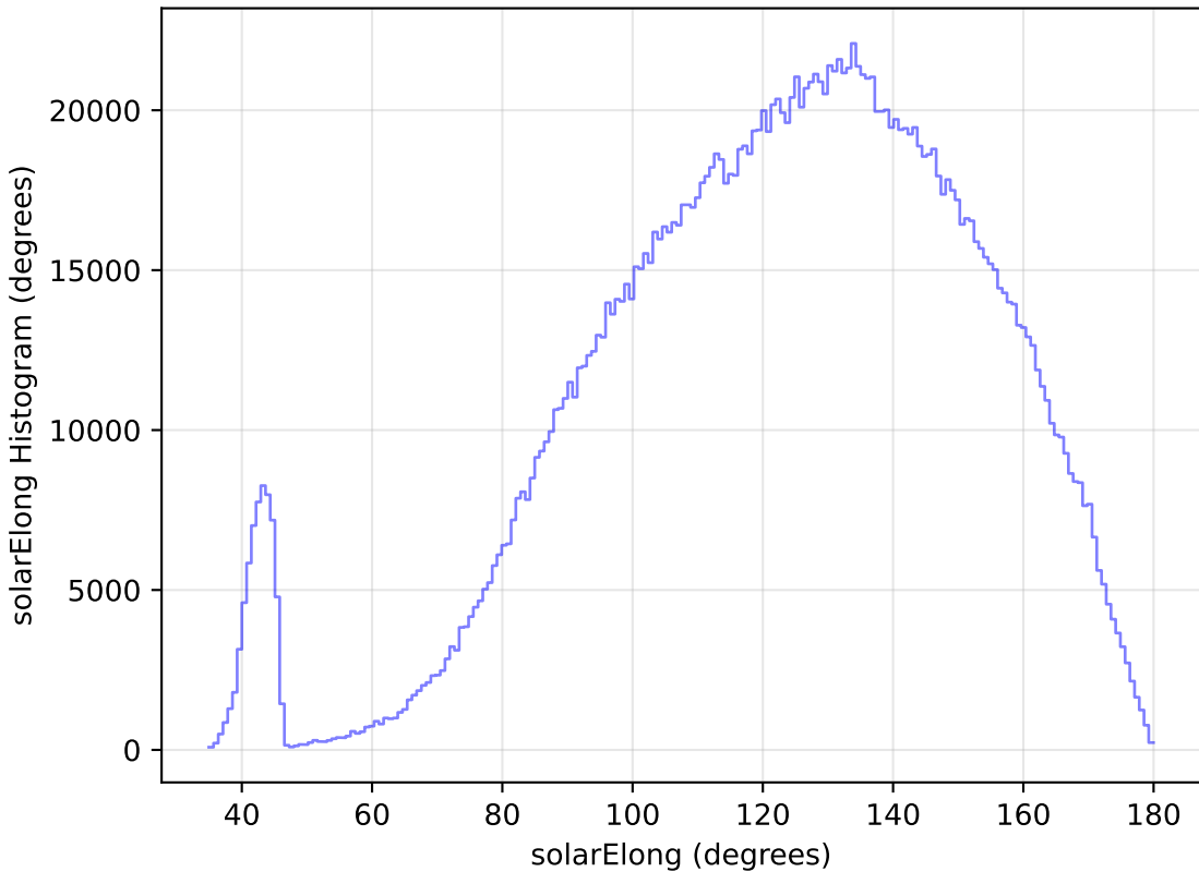
ddf_loaded_half_fl4_v3.4_10yrs All sky all bands: solarElong Histogram
