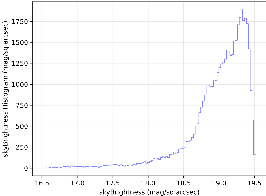
ddf_loaded_half_fl4_v3.4_10yrs Yr 1 z band: skyBrightness Histogram
