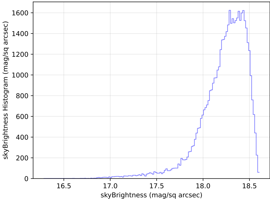
ddf_loaded_half_fl4_v3.4_10yrs Yr 1 y band: skyBrightness Histogram
