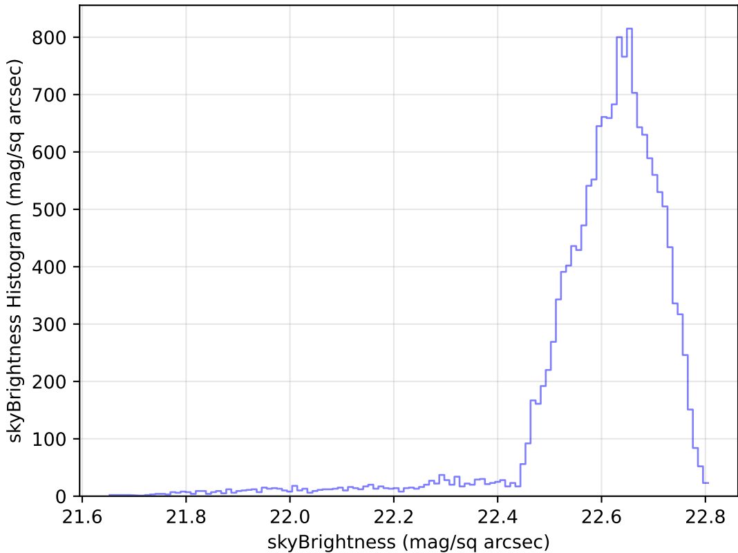
ddf_loaded_half_fl4_v3.4_10yrs Yr 1 u band: skyBrightness Histogram
