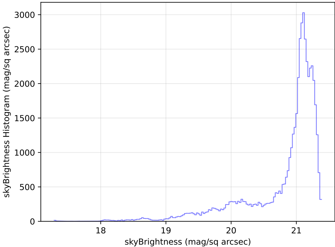
ddf_loaded_half_fl4_v3.4_10yrs Yr 1 r band: skyBrightness Histogram
