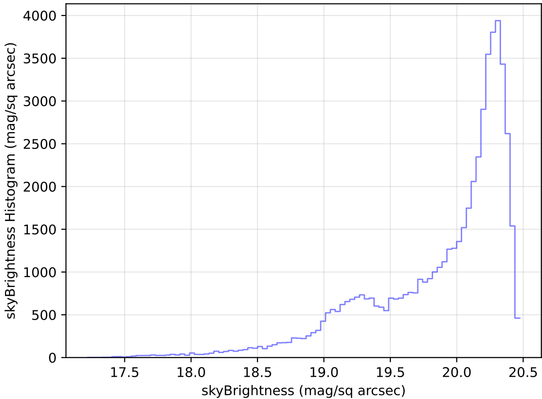
ddf_loaded_half_fl4_v3.4_10yrs Yr 1 i band: skyBrightness Histogram
