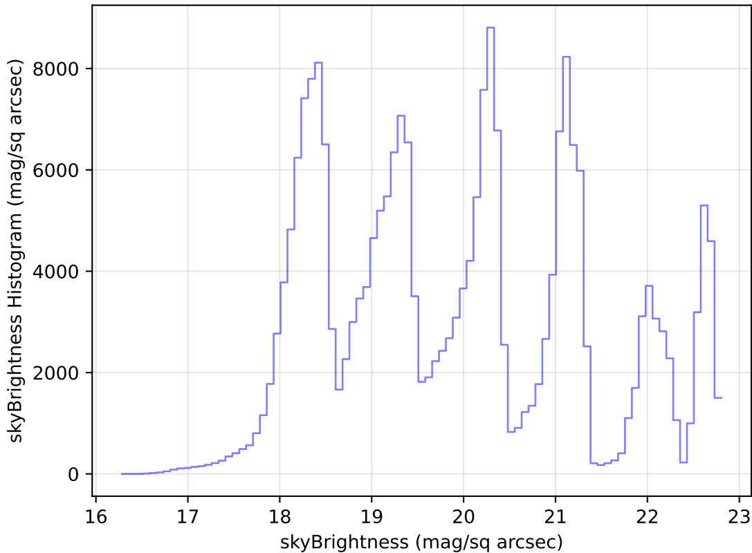
ddf_loaded_half_fl4_v3.4_10yrs Yr 1 all bands: skyBrightness Histogram
