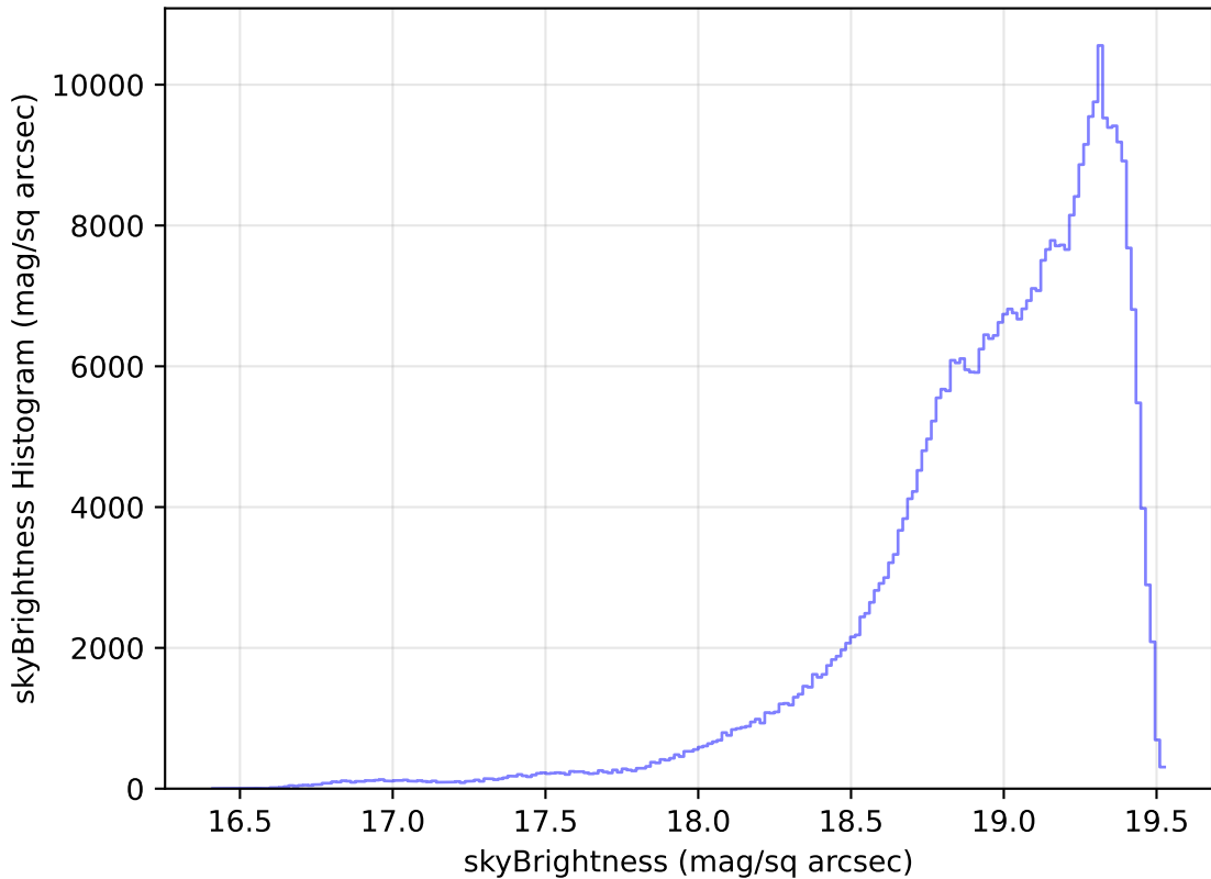
ddf_loaded_half_fl4_v3.4_10yrs WFD z band: skyBrightness Histogram
