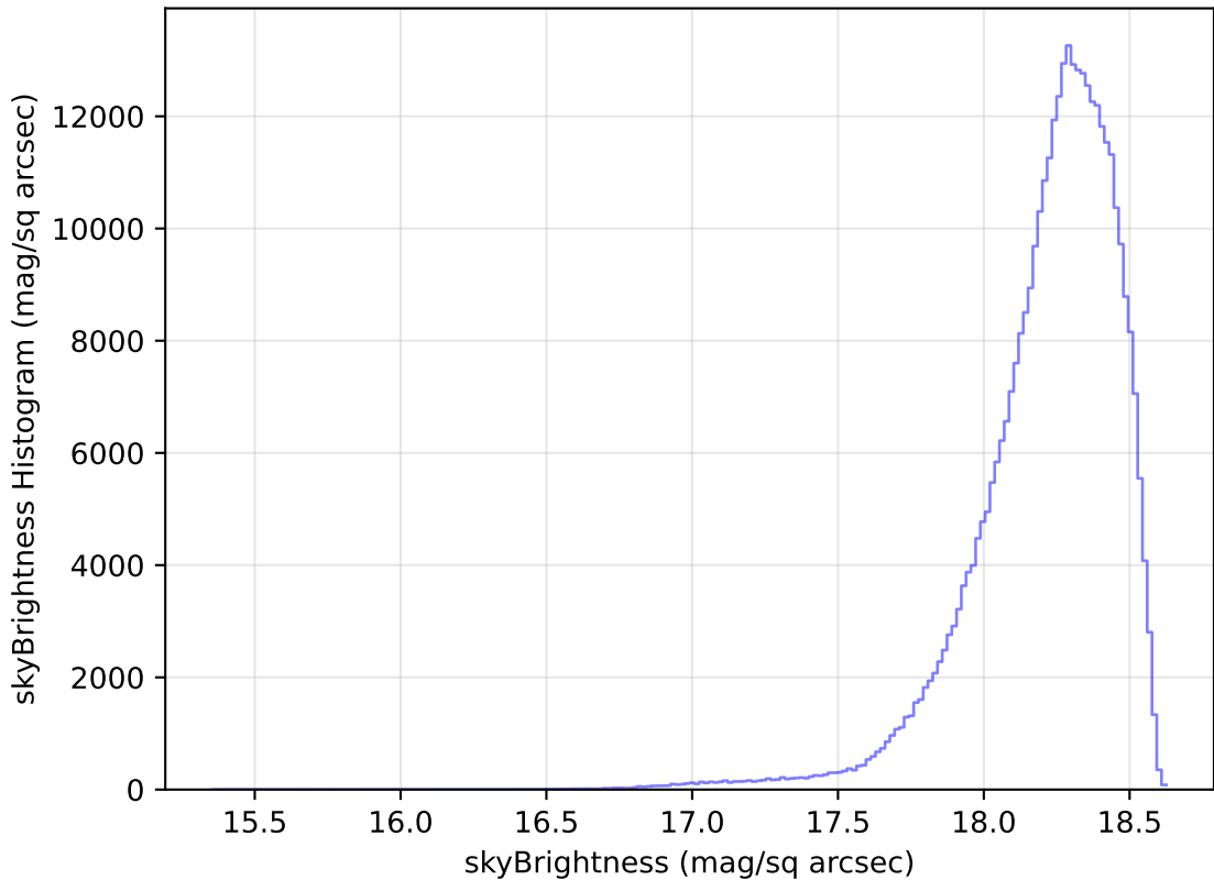
ddf_loaded_half_fl4_v3.4_10yrs WFD y band: skyBrightness Histogram
