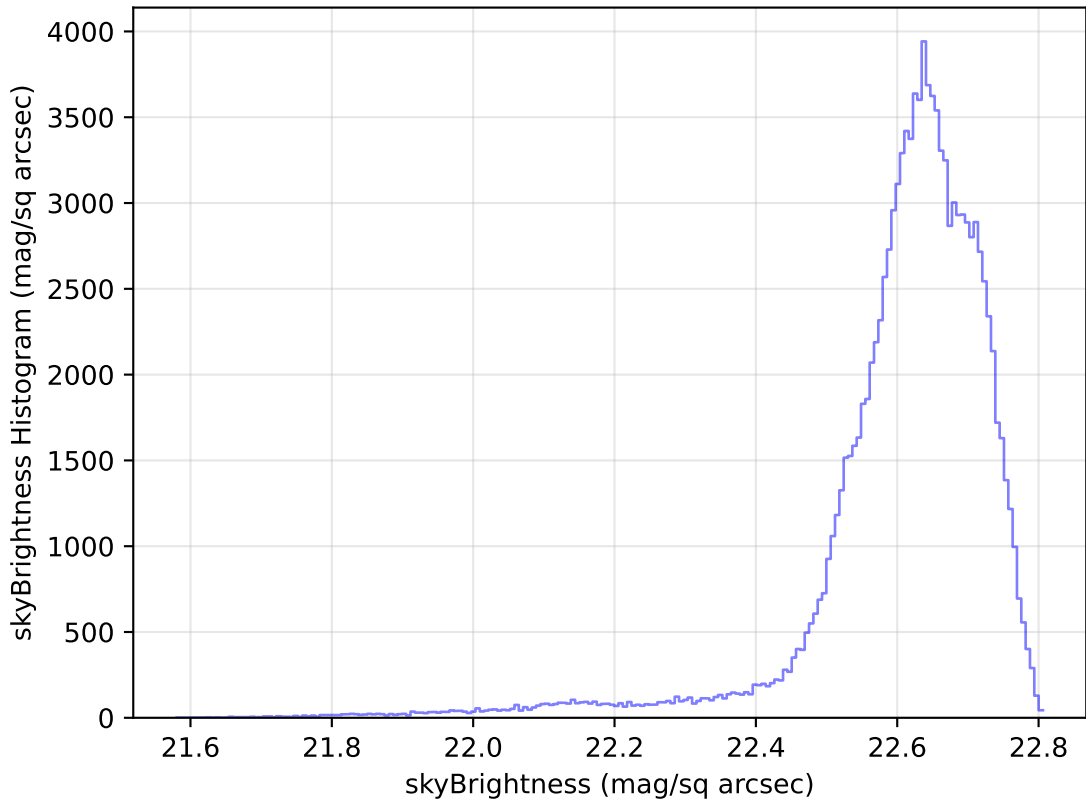
ddf_loaded_half_fl4_v3.4_10yrs WFD u band: skyBrightness Histogram
