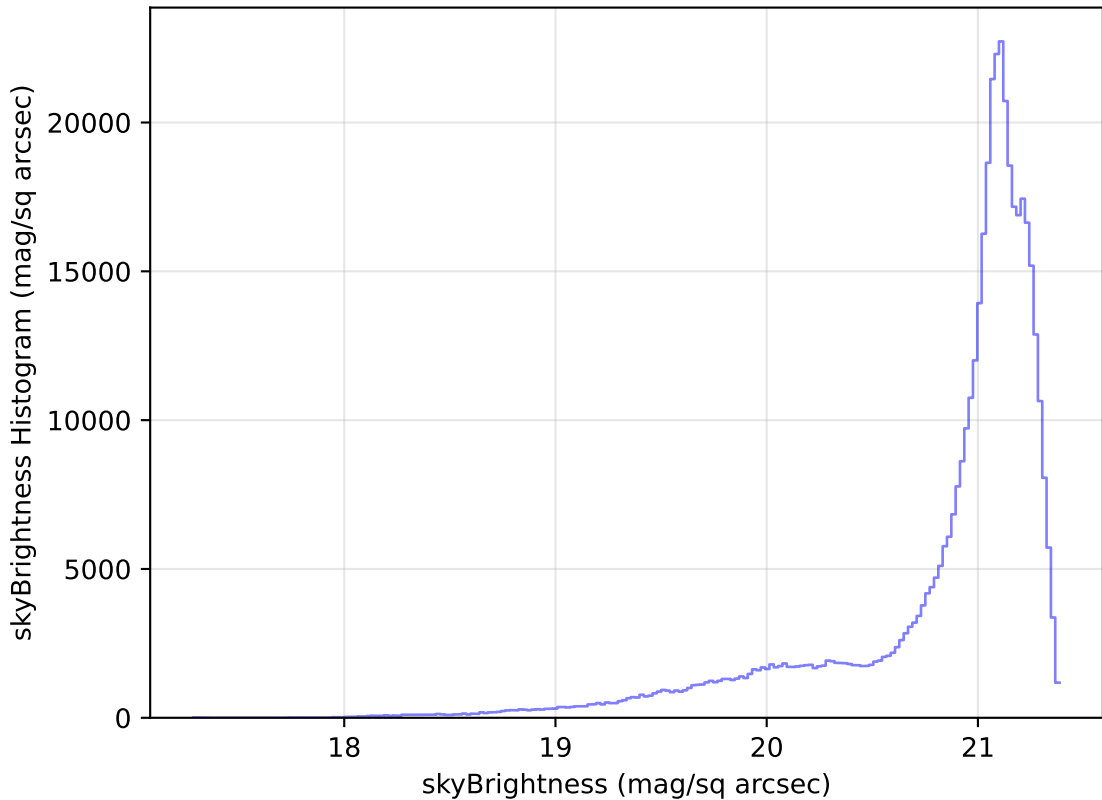
ddf_loaded_half_fl4_v3.4_10yrs WFD r band: skyBrightness Histogram
