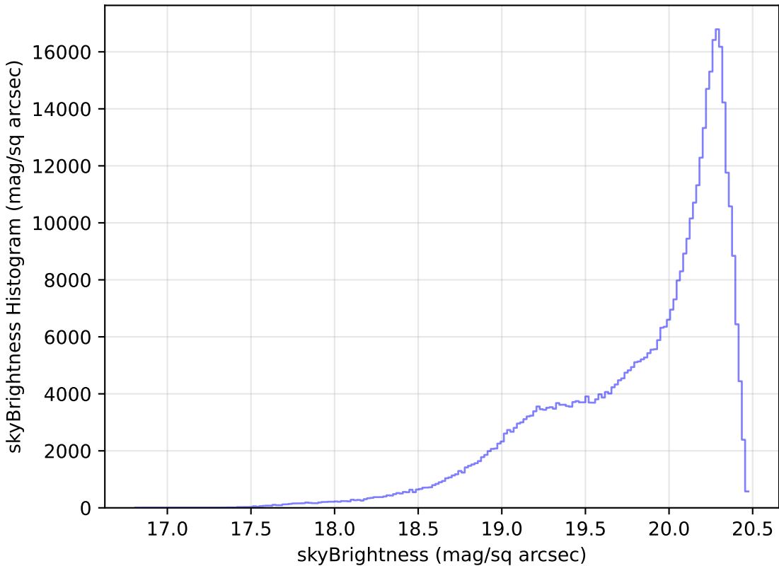
ddf_loaded_half_fl4_v3.4_10yrs WFD i band: skyBrightness Histogram
