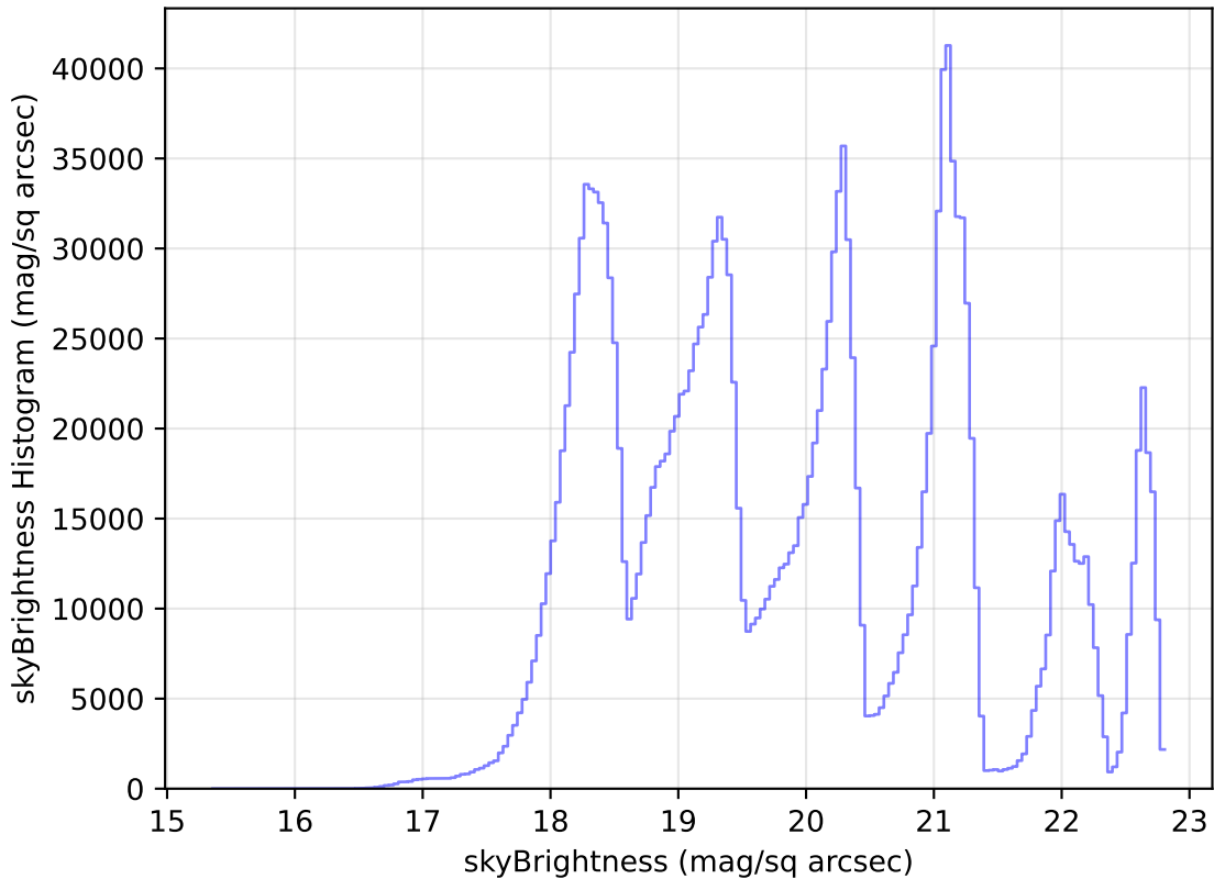
ddf_loaded_half_fl4_v3.4_10yrs WFD all bands: skyBrightness Histogram
