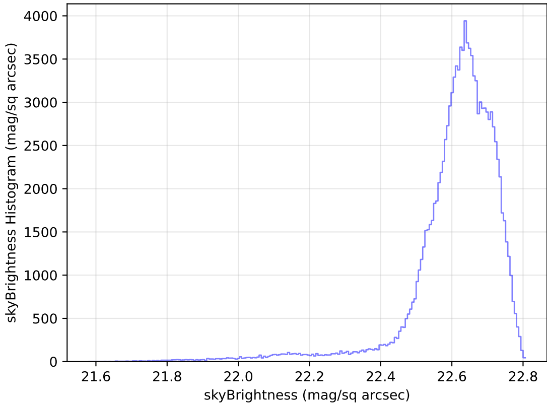
ddf_loaded_half_fl4_v3.4_10yrs All sky u band: skyBrightness Histogram
