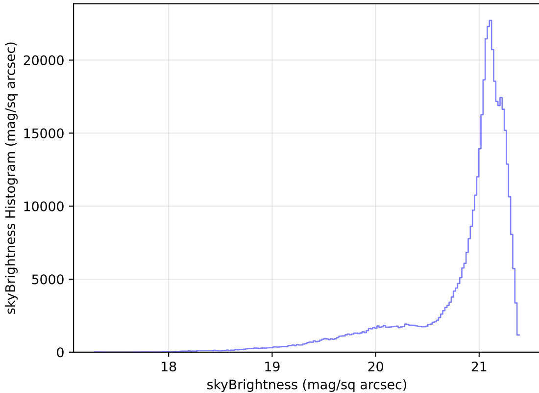
ddf_loaded_half_fl4_v3.4_10yrs All sky r band: skyBrightness Histogram
