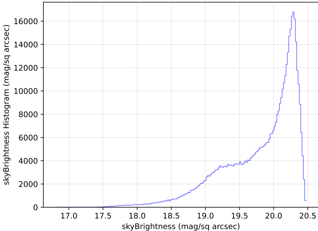
ddf_loaded_half_fl4_v3.4_10yrs All sky i band: skyBrightness Histogram
