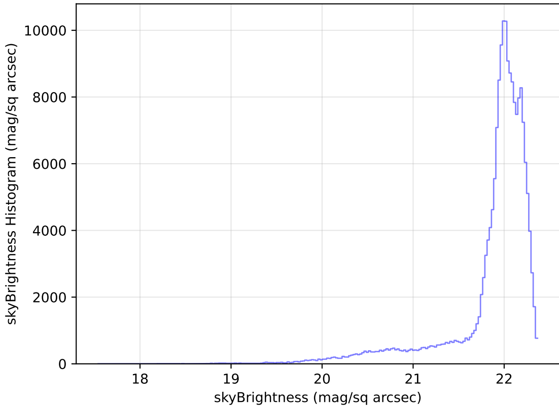
ddf_loaded_half_fl4_v3.4_10yrs All sky g band: skyBrightness Histogram
