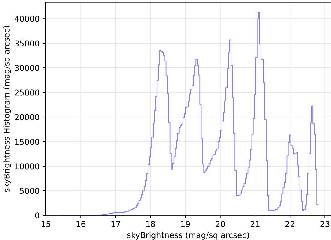
ddf_loaded_half_fl4_v3.4_10yrs All sky all bands: skyBrightness Histogram
