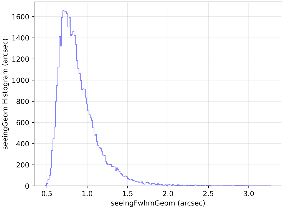
ddf_loaded_half_fl4_v3.4_10yrs Yr 1 z band: seeingGeom Histogram
