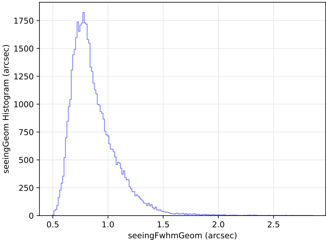
ddf_loaded_half_fl4_v3.4_10yrs Yr 1 y band: seeingGeom Histogram
