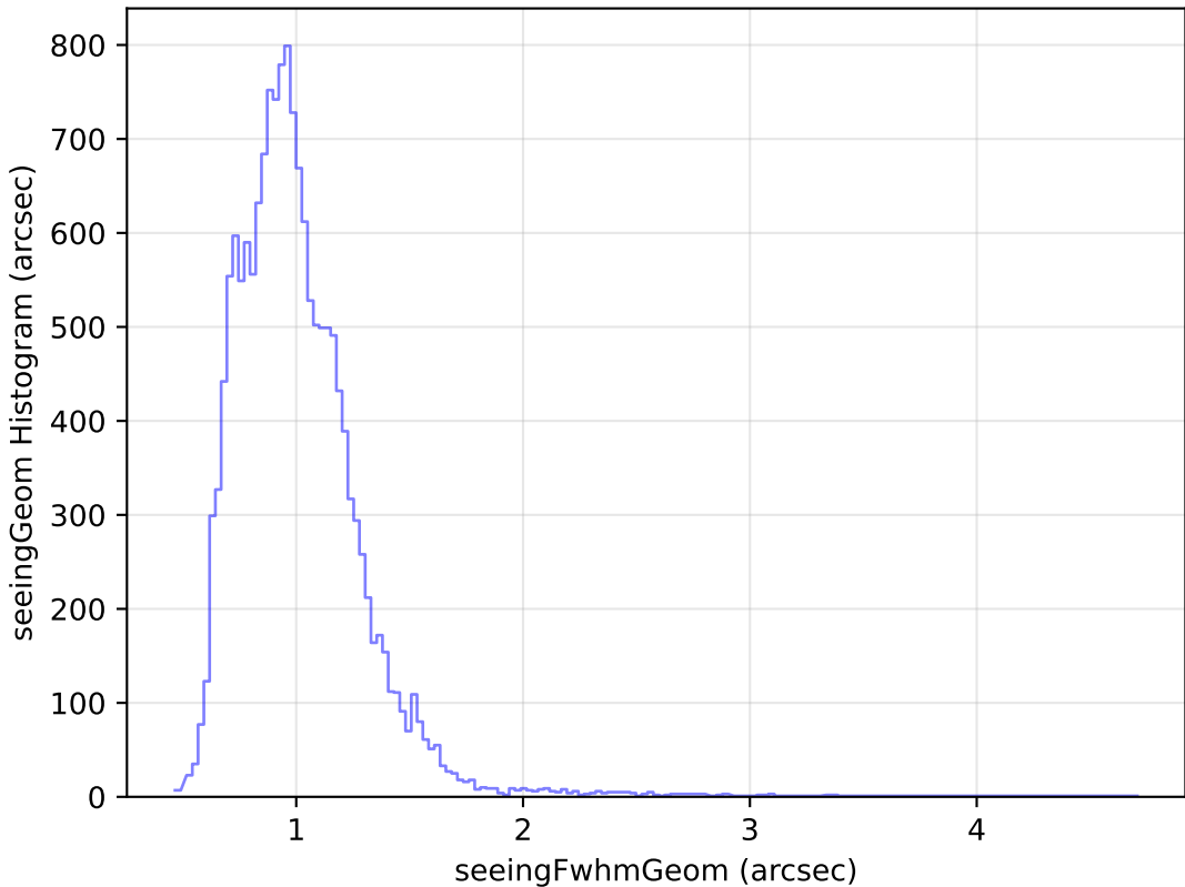
ddf_loaded_half_fl4_v3.4_10yrs Yr 1 u band: seeingGeom Histogram
