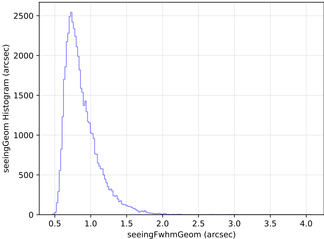
ddf_loaded_half_fl4_v3.4_10yrs Yr 1 r band: seeingGeom Histogram
