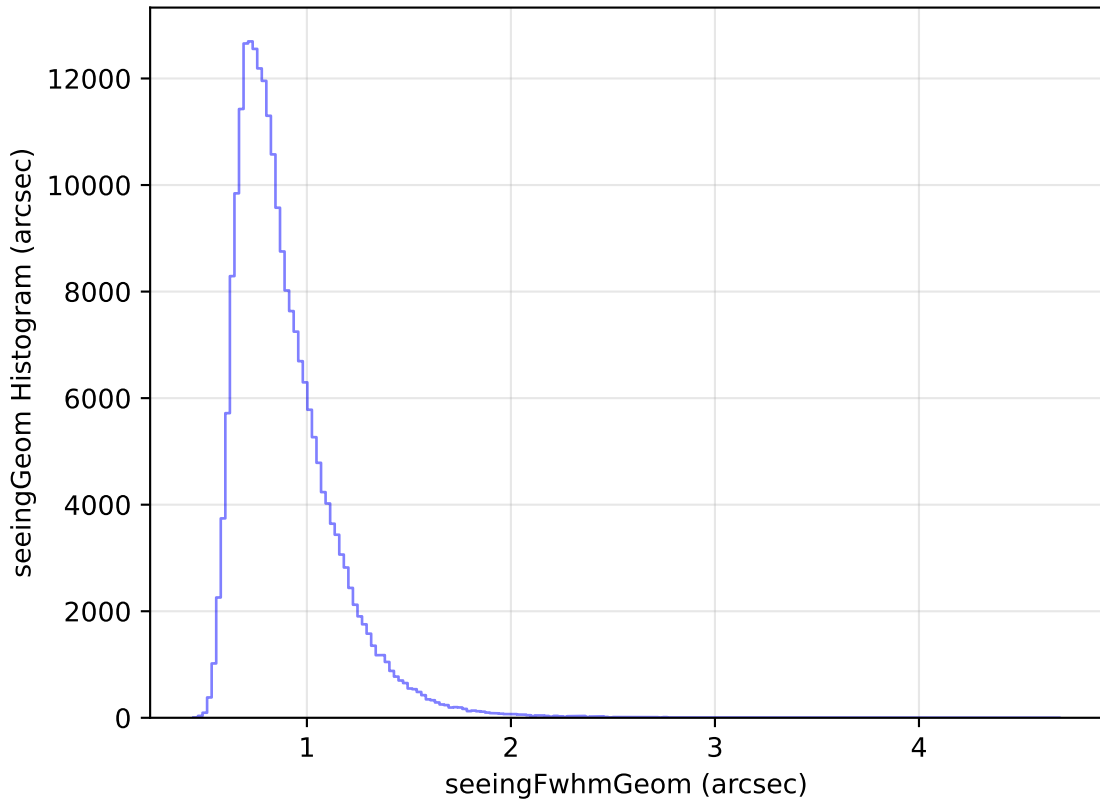
ddf_loaded_half_fl4_v3.4_10yrs Yr 1 all bands: seeingGeom Histogram
