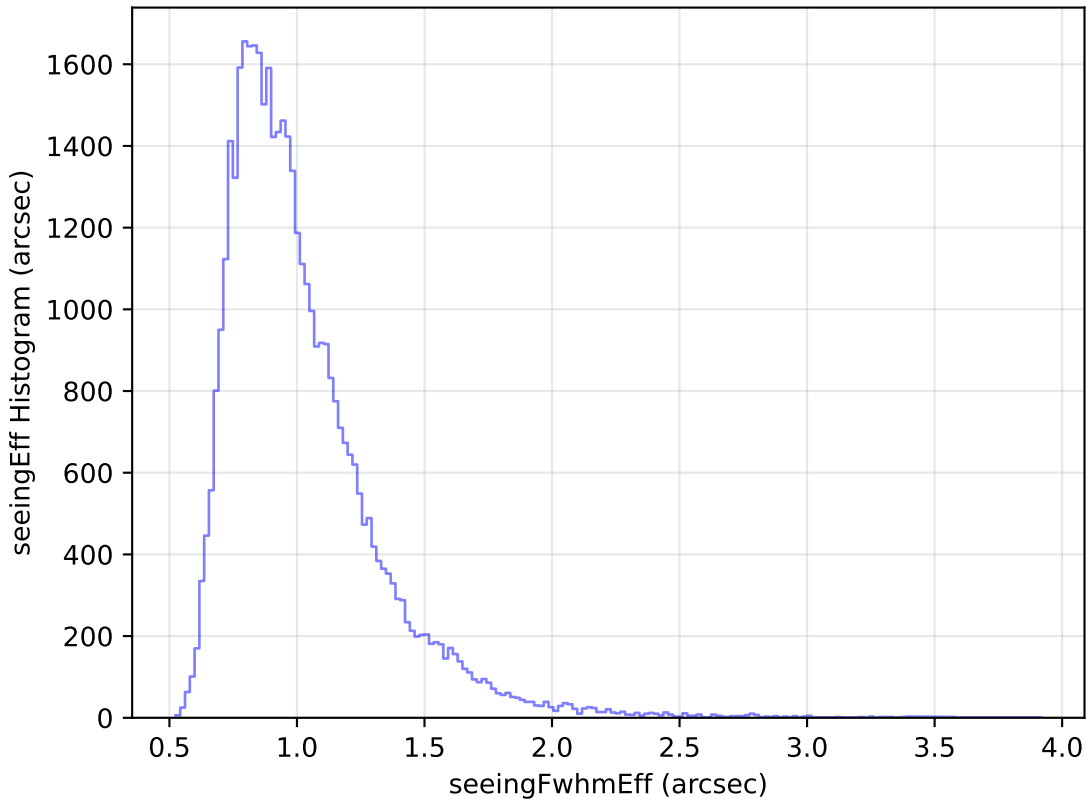
ddf_loaded_half_fl4_v3.4_10yrs Yr 1 z band: seeingEff Histogram
