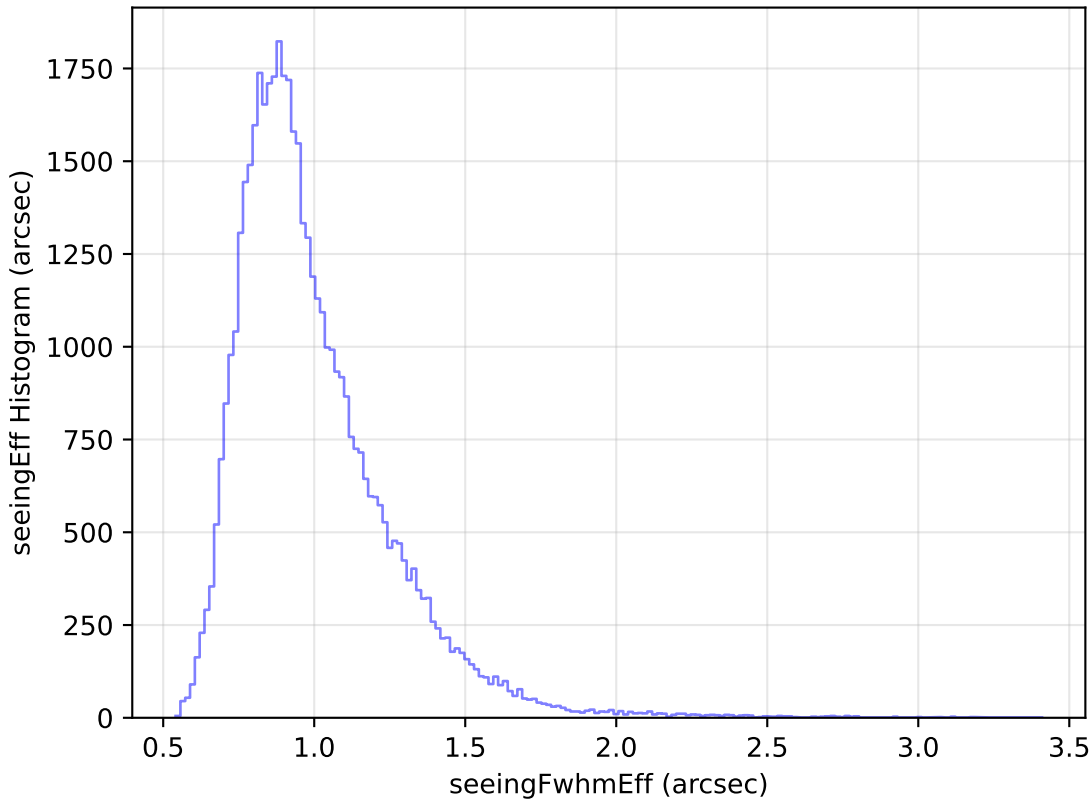
ddf_loaded_half_fl4_v3.4_10yrs Yr 1 y band: seeingEff Histogram
