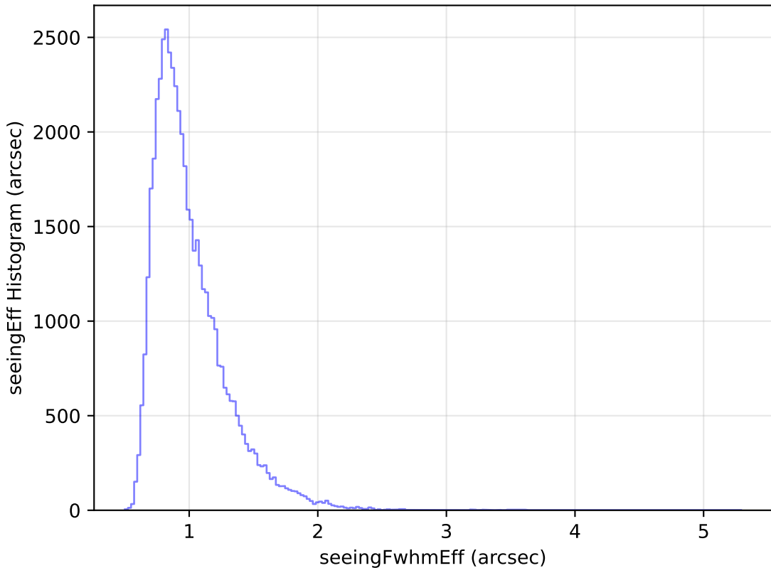
ddf_loaded_half_fl4_v3.4_10yrs Yr 1 r band: seeingEff Histogram
