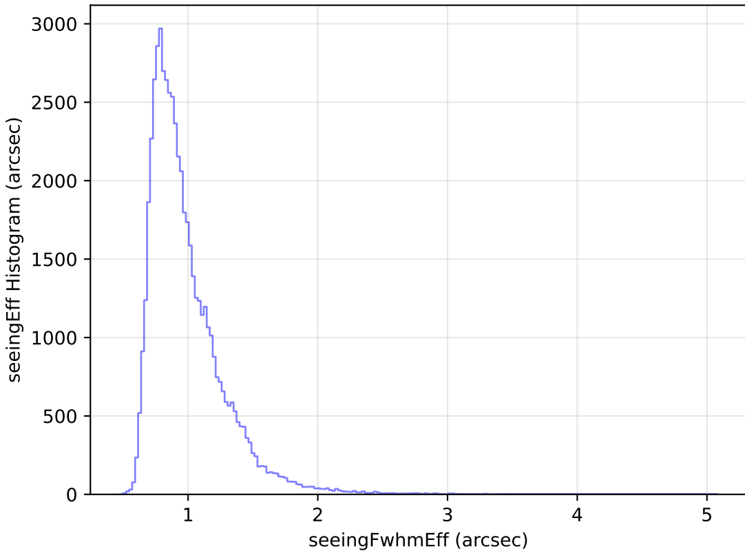
ddf_loaded_half_fl4_v3.4_10yrs Yr 1 i band: seeingEff Histogram
