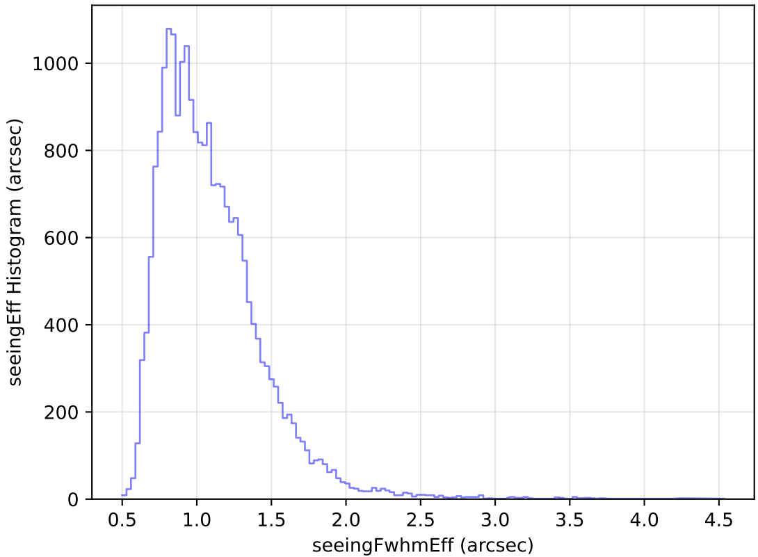
ddf_loaded_half_fl4_v3.4_10yrs Yr 1 g band: seeingEff Histogram
