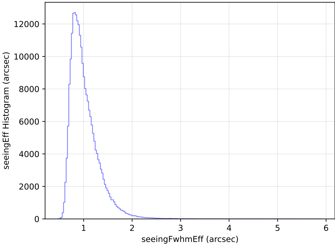
ddf_loaded_half_fl4_v3.4_10yrs Yr 1 all bands: seeingEff Histogram
