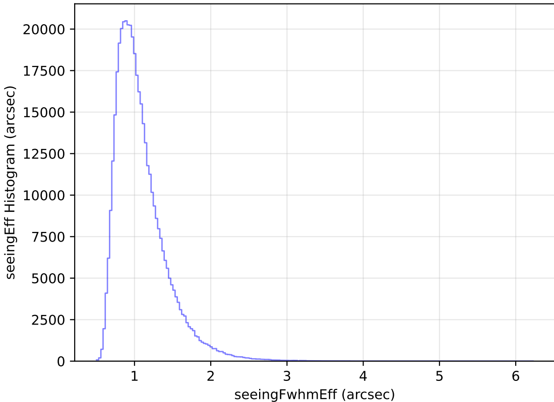
ddf_loaded_half_fl4_v3.4_10yrs WFD z band: seeingEff Histogram
