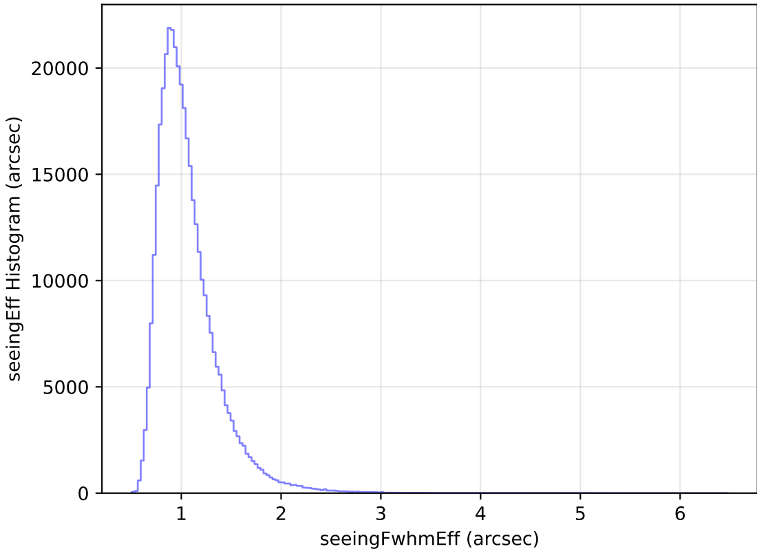
ddf_loaded_half_fl4_v3.4_10yrs WFD y band: seeingEff Histogram
