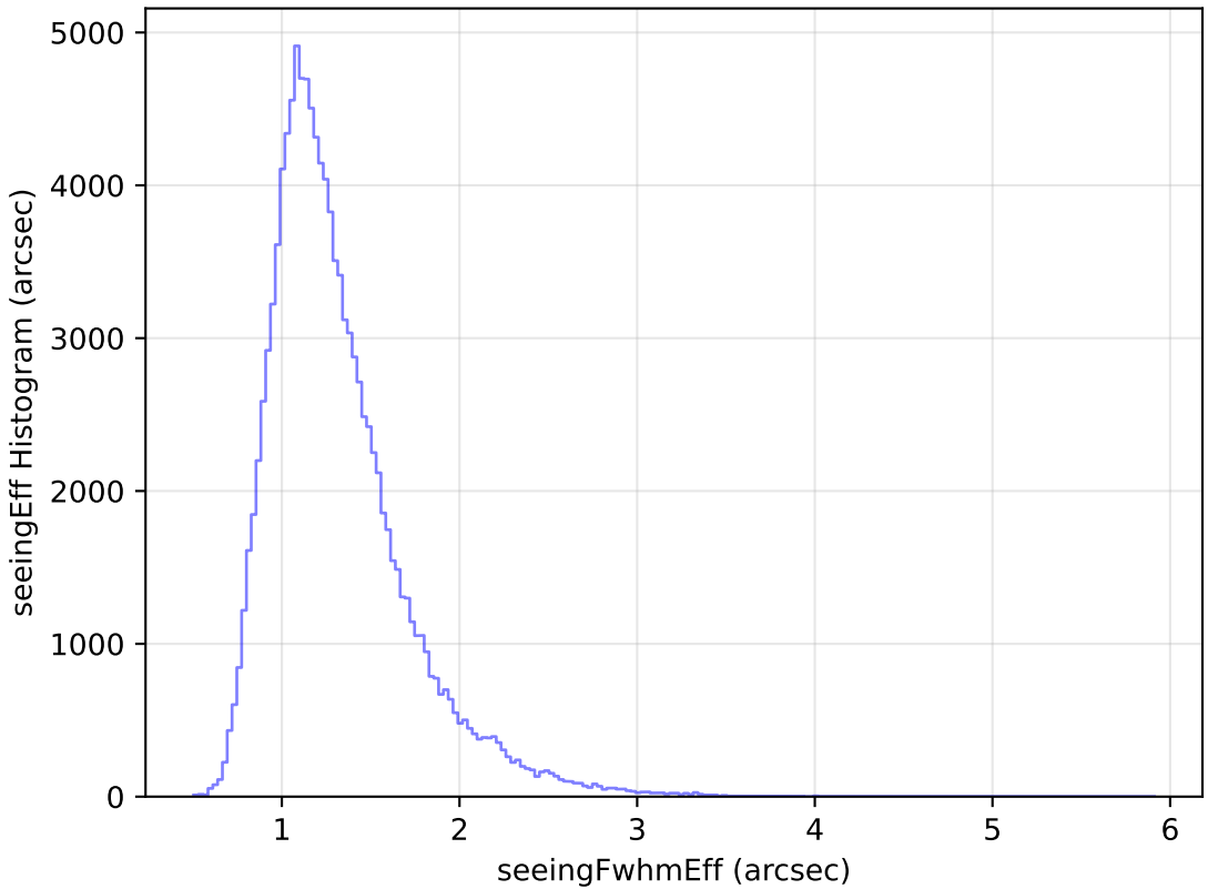
ddf_loaded_half_fl4_v3.4_10yrs WFD u band: seeingEff Histogram
