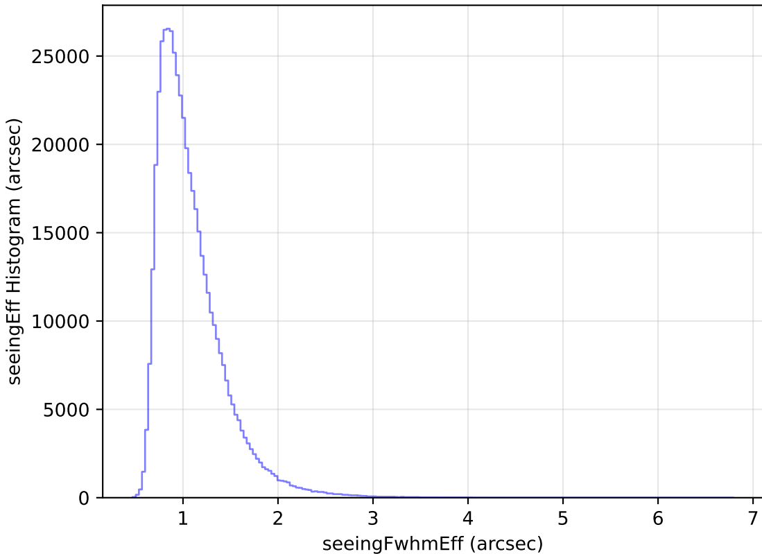
ddf_loaded_half_fl4_v3.4_10yrs WFD i band: seeingEff Histogram
