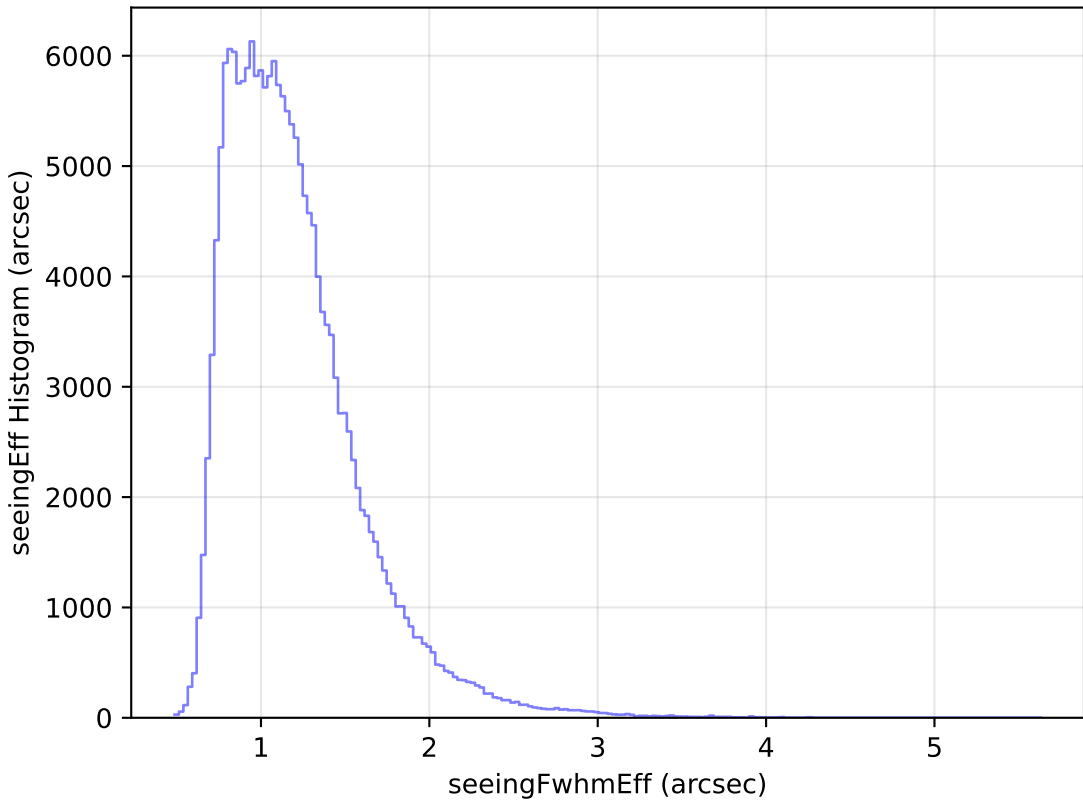
ddf_loaded_half_fl4_v3.4_10yrs WFD g band: seeingEff Histogram
