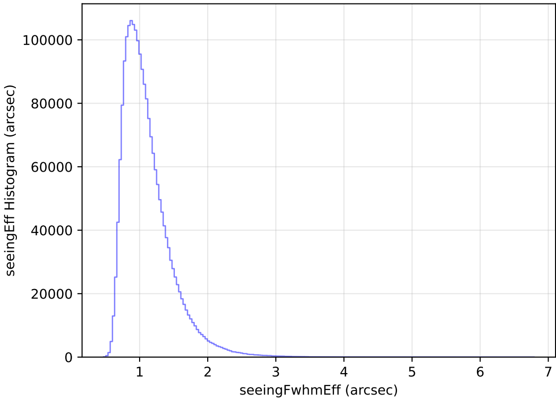
ddf_loaded_half_fl4_v3.4_10yrs WFD all bands: seeingEff Histogram
