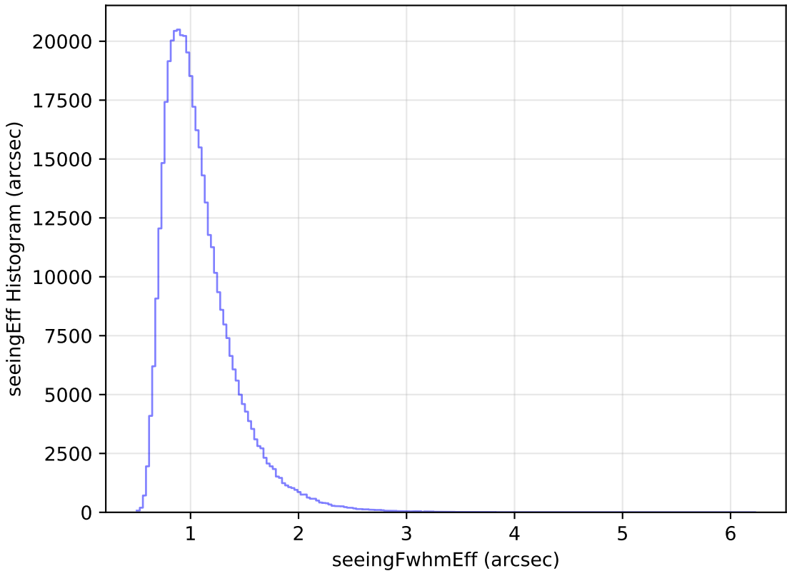
ddf_loaded_half_fl4_v3.4_10yrs All sky z band: seeingEff Histogram
