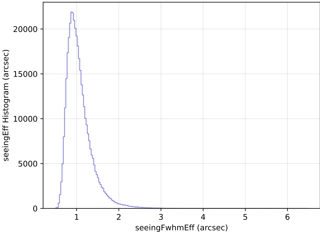
ddf_loaded_half_fl4_v3.4_10yrs All sky y band: seeingEff Histogram
