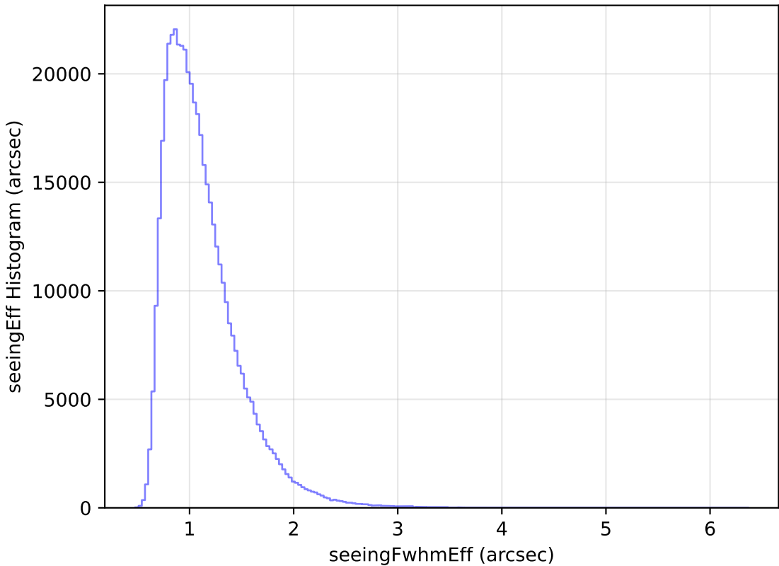
ddf_loaded_half_fl4_v3.4_10yrs All sky r band: seeingEff Histogram
