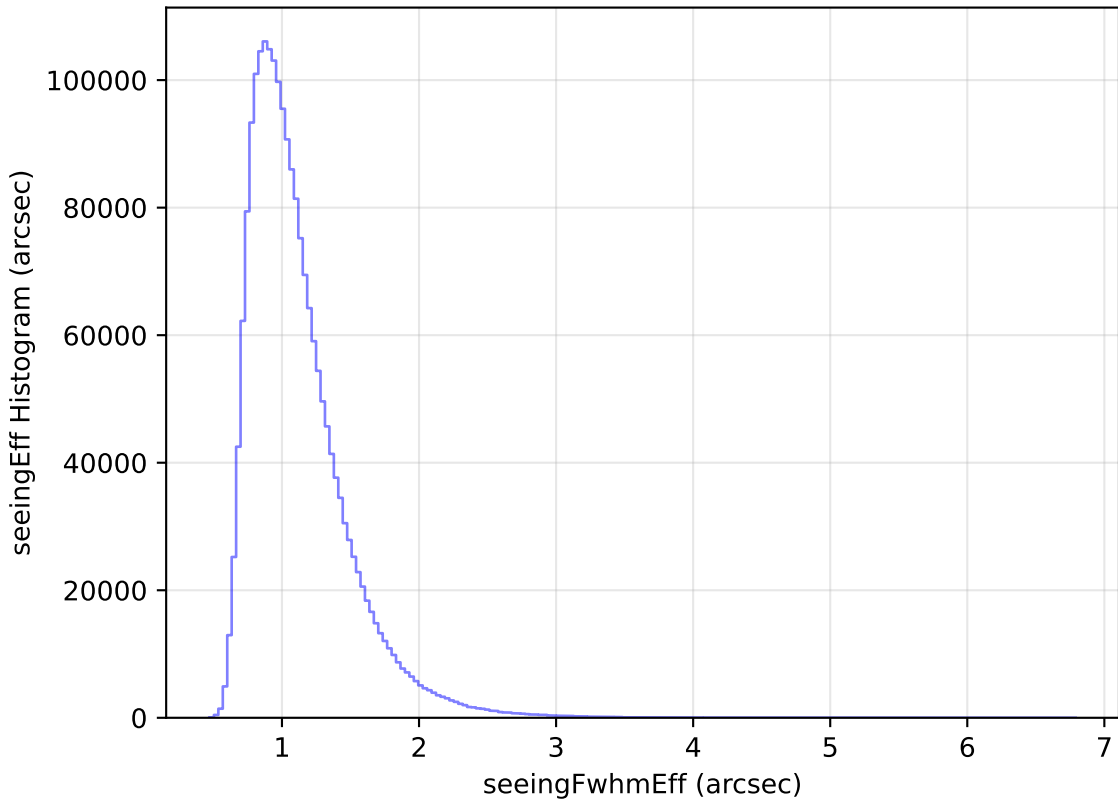
ddf_loaded_half_fl4_v3.4_10yrs All sky all bands: seeingEff Histogram
