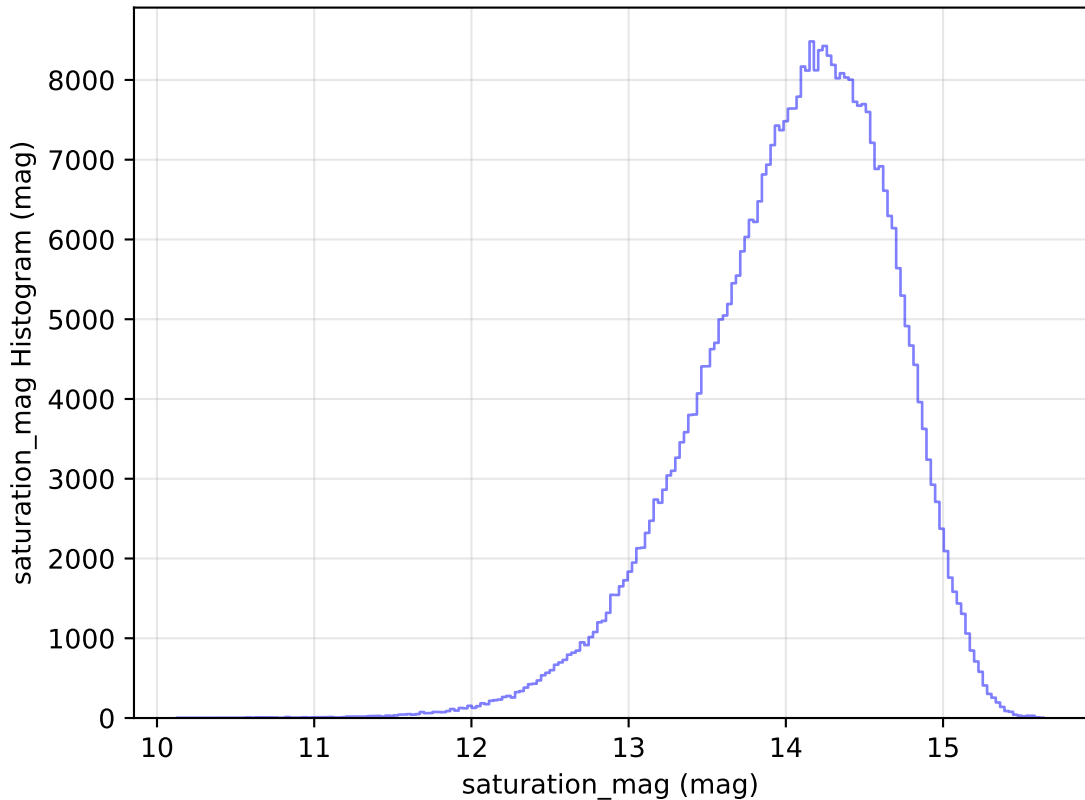
ddf_loaded_half_fl4_v3.4_10yrs WFD z band: saturation_mag Histogram
