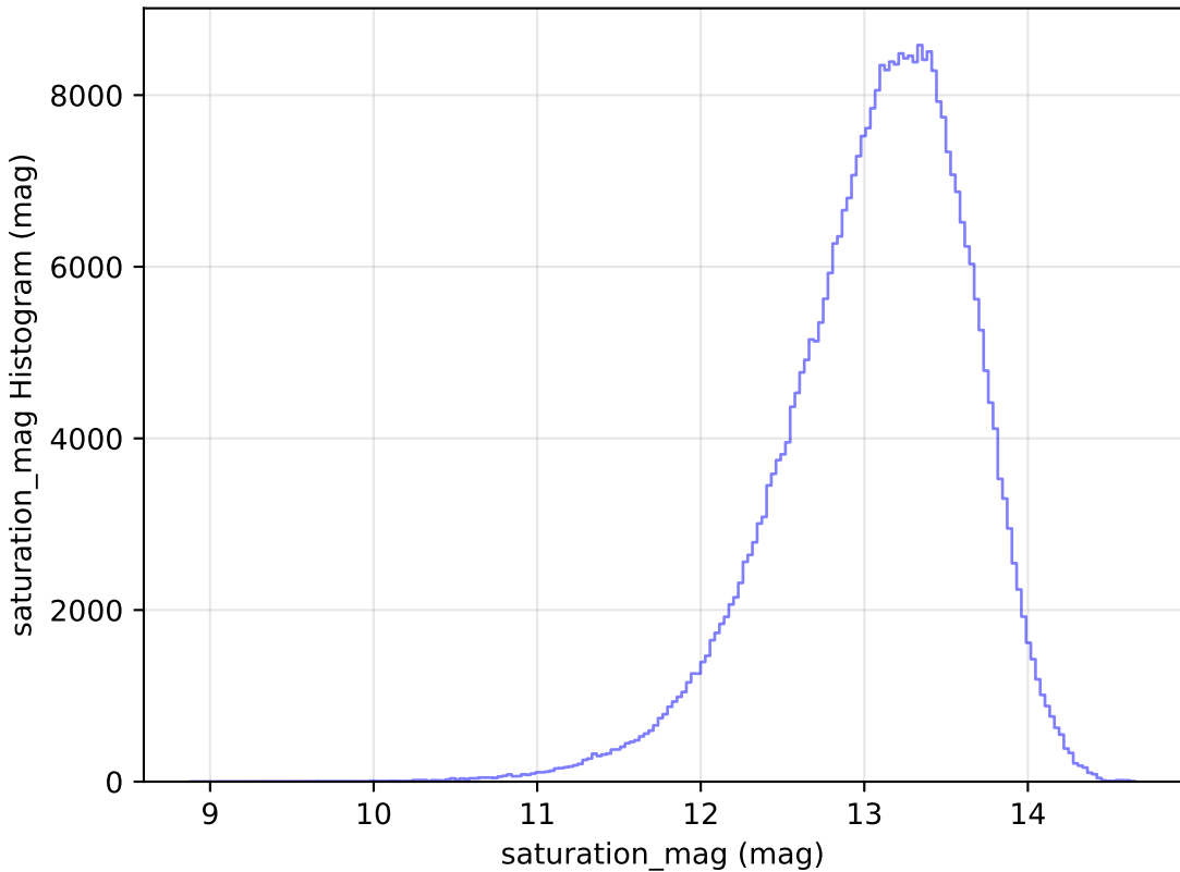
ddf_loaded_half_fl4_v3.4_10yrs WFD y band: saturation_mag Histogram
