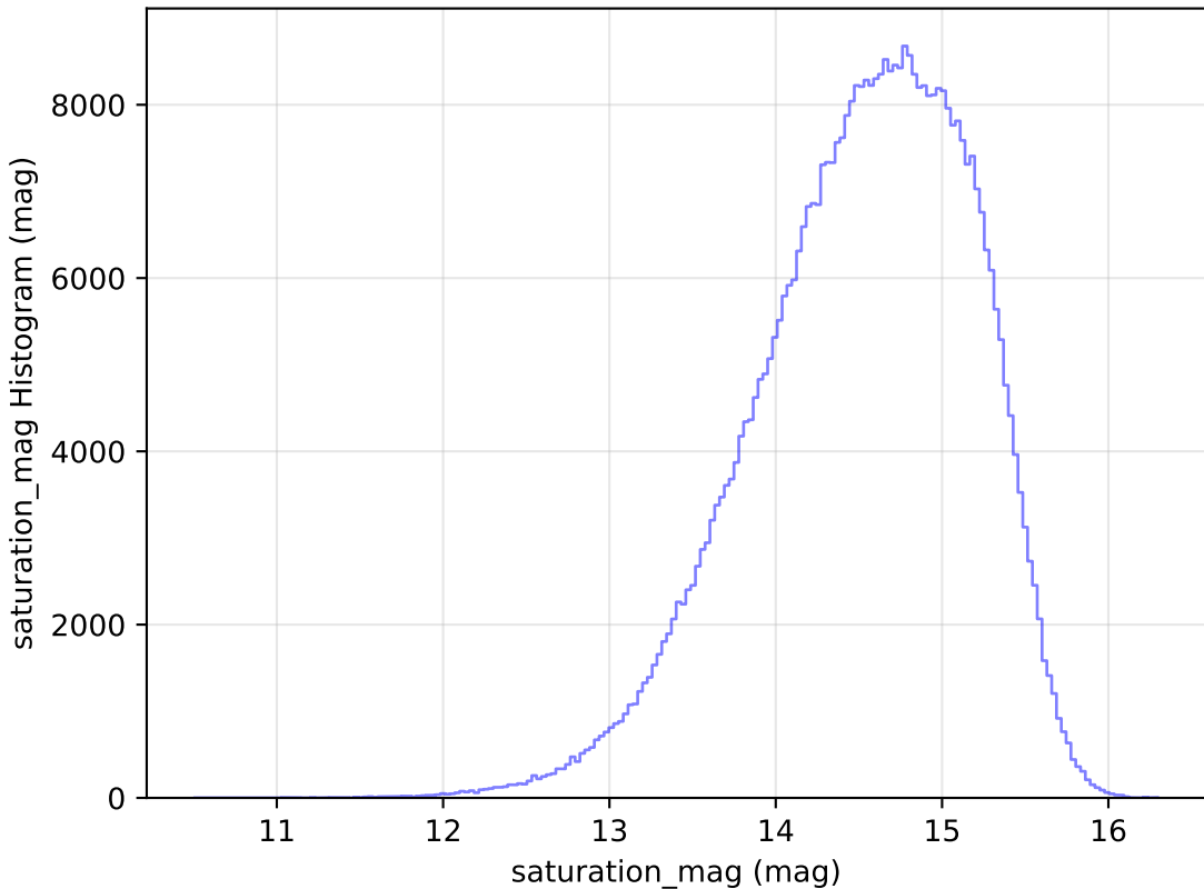
ddf_loaded_half_fl4_v3.4_10yrs WFD r band: saturation_mag Histogram
