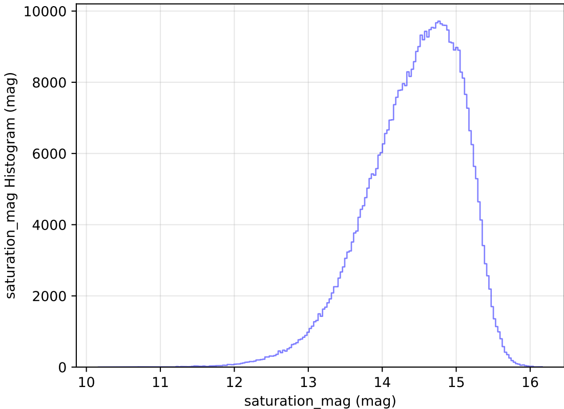
ddf_loaded_half_fl4_v3.4_10yrs WFD i band: saturation_mag Histogram
