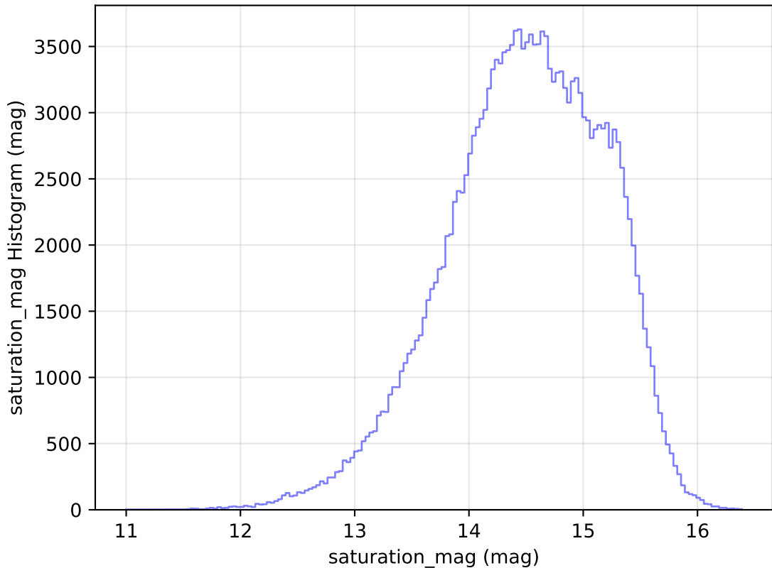
ddf_loaded_half_fl4_v3.4_10yrs WFD g band: saturation_mag Histogram
