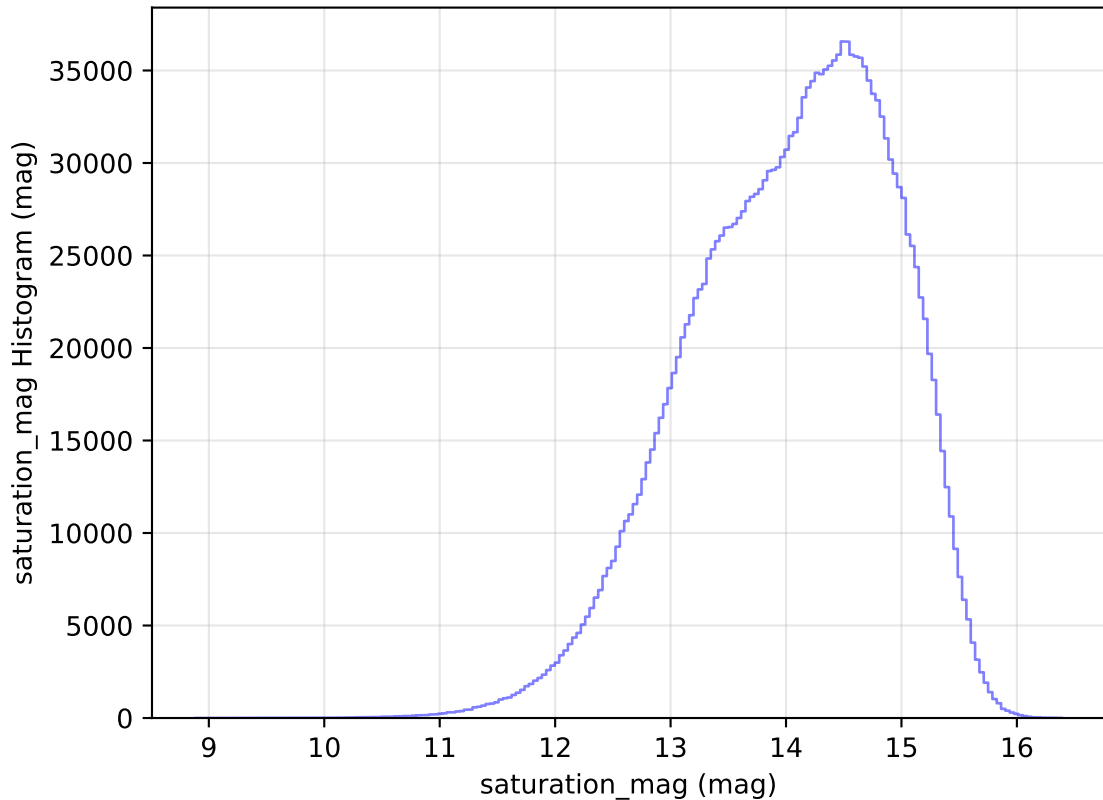
ddf_loaded_half_fl4_v3.4_10yrs WFD all bands: saturation_mag Histogram
