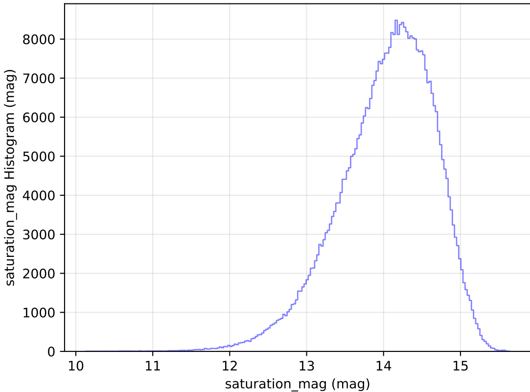
ddf_loaded_half_fl4_v3.4_10yrs All sky z band: saturation_mag Histogram
