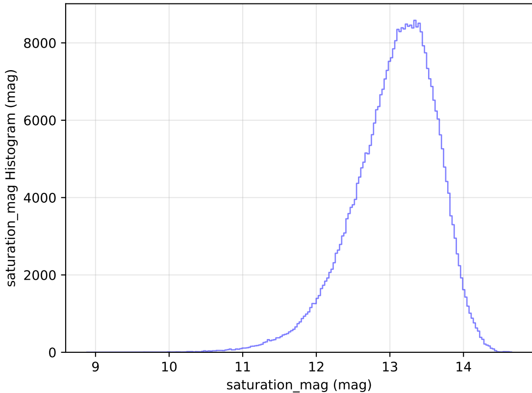
ddf_loaded_half_fl4_v3.4_10yrs All sky y band: saturation_mag Histogram
