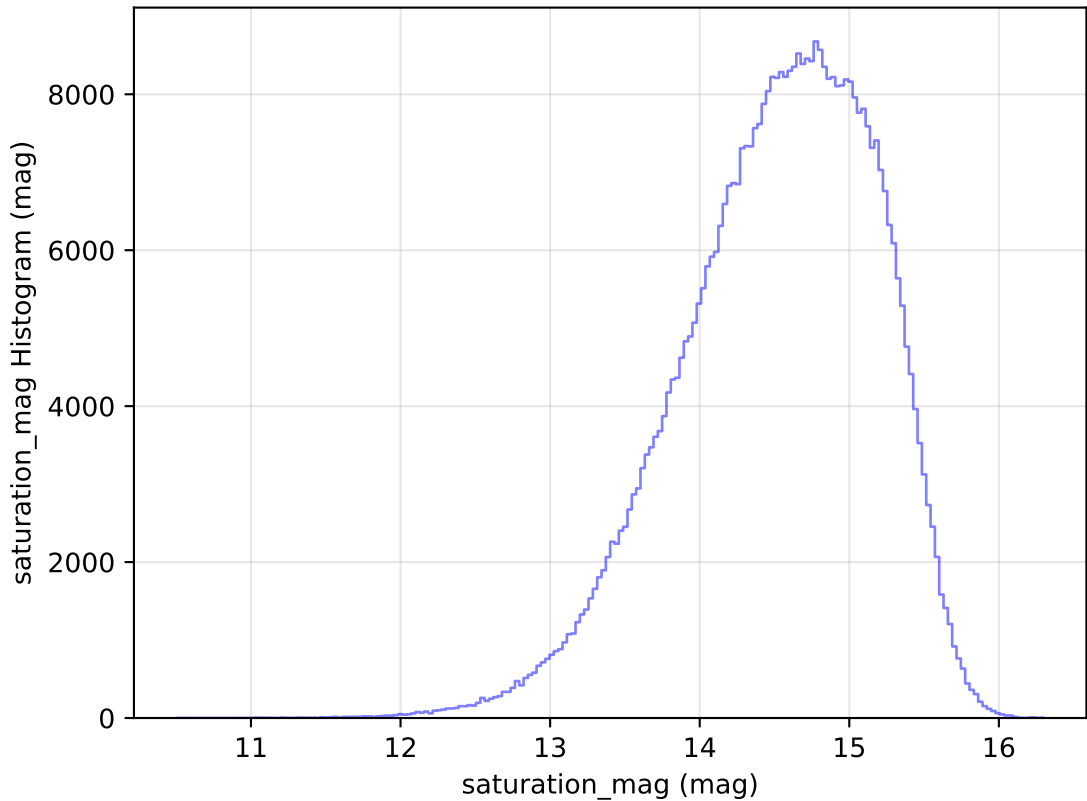
ddf_loaded_half_fl4_v3.4_10yrs All sky r band: saturation_mag Histogram
